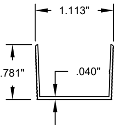
13 SASH STOP 6063-T6 ALUMINUM
