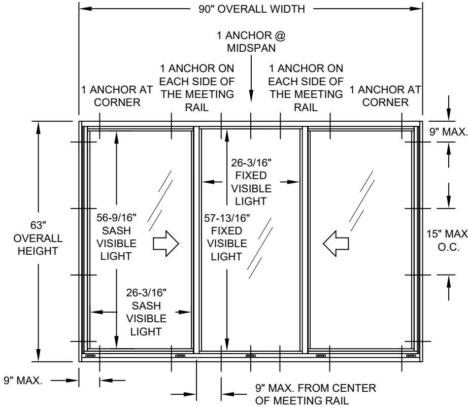
TYP. XO (1/3-1/3-1/3) ANCHORAGE & MAX. VISIBLE LIGHT OPENING
