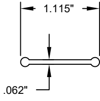
12 DOGBONE REINFORCEMENT 6063-T6 ALUMINUM
