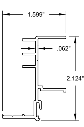
4 FRAME JAMB (FIXED) 6063-T6 ALUMINUM
