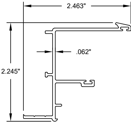
5 FRAME JAMB (OPERABLE) 6063-T6 ALUMINUM
