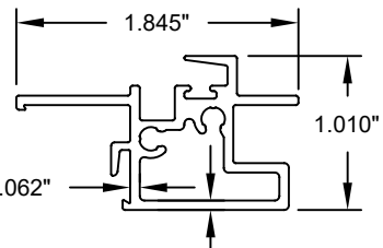
9 STD. MEETING RAIL 6063-T6 ALUMINUM
