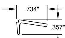
17 IG BEADING PVC
