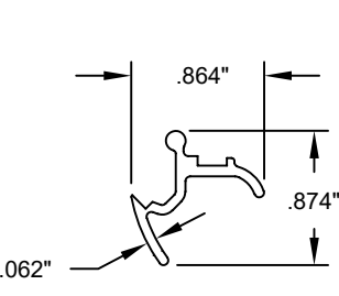
7 SIDE RAIL LOCK 6063-T6 ALUMINUM
