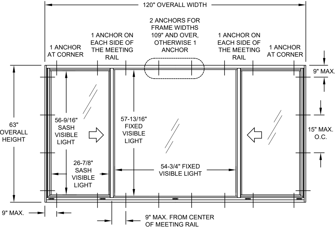
TYP. XO (1/4-1/2-1/4) ANCHORAGE & MAX. VISIBLE LIGHT OPENING
